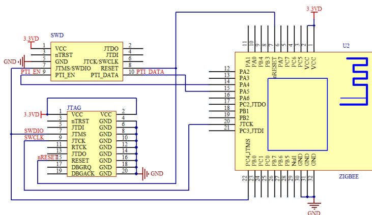
Figure 3-22. SWD connection
