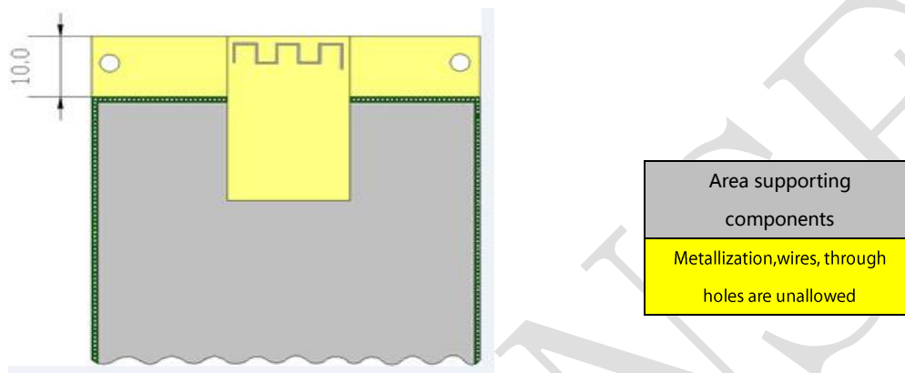
Figure 3-13. PCB Layout of the Proposed Antenna Selection
